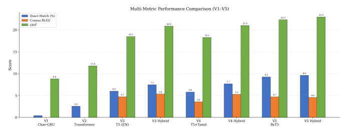
Fig. 2. Multi-metric comparison (EM, BLEU, chrF) across all model versions.
